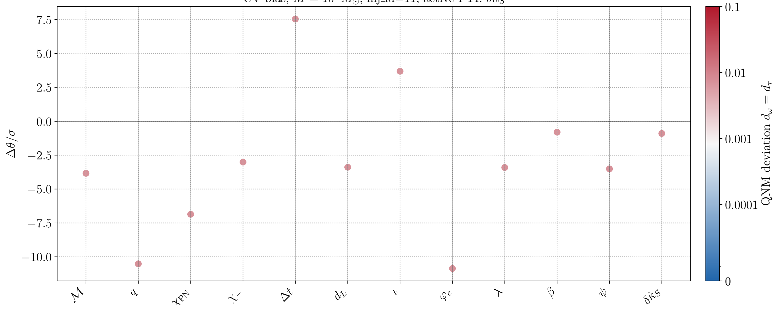
CV bias, M = 10^6 M_\odot , inj_id=11, active FTL: \delta\hat{\kappa}_S
