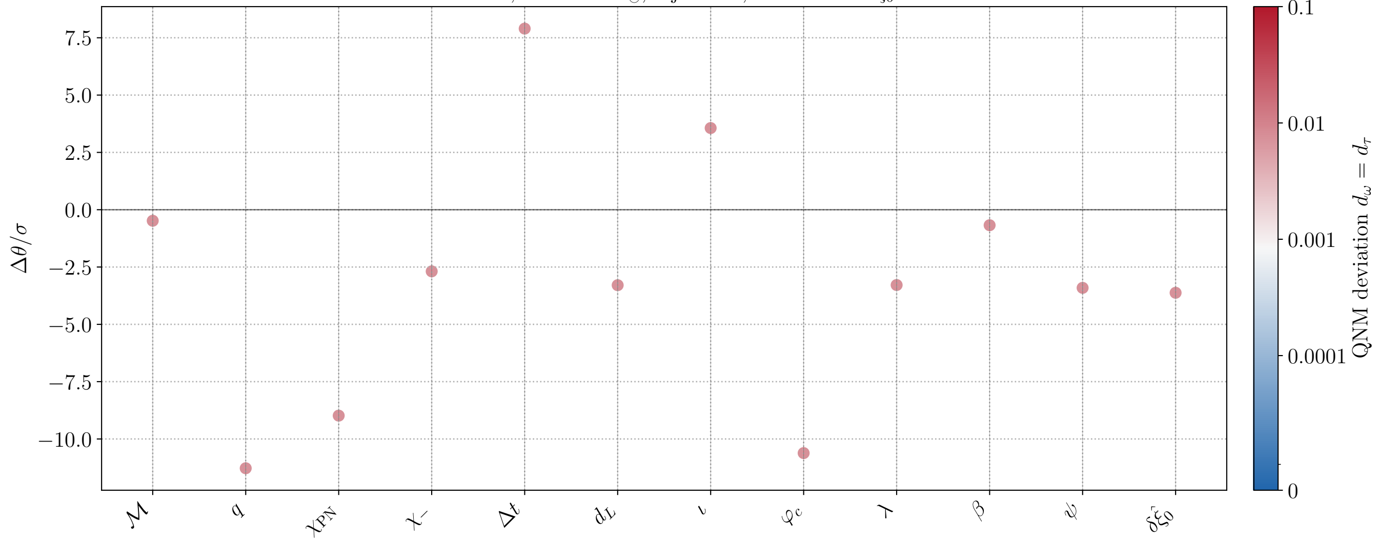
CV bias, M = 10^6 M_\odot , inj_id=11, active FTI: \delta\hat{\xi}_0
