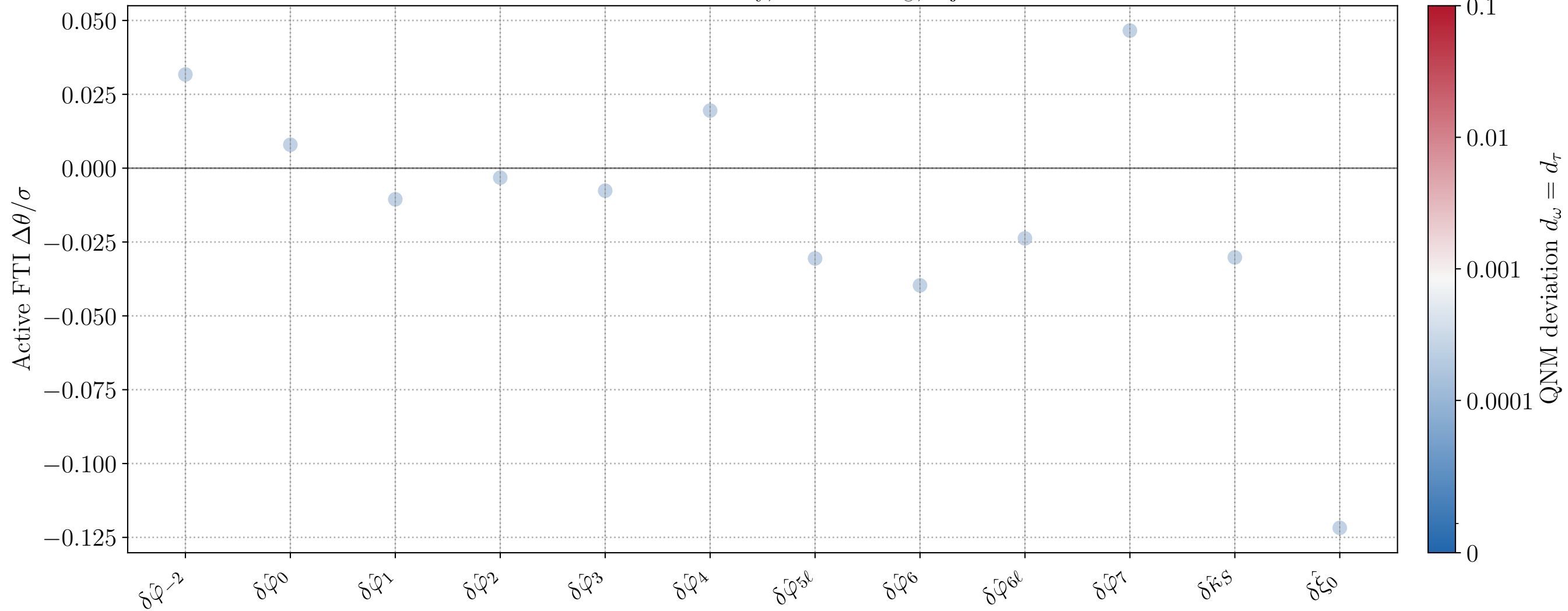
Active-FTI bias summary, M = 10^6 M_\odot , inj_id=12
