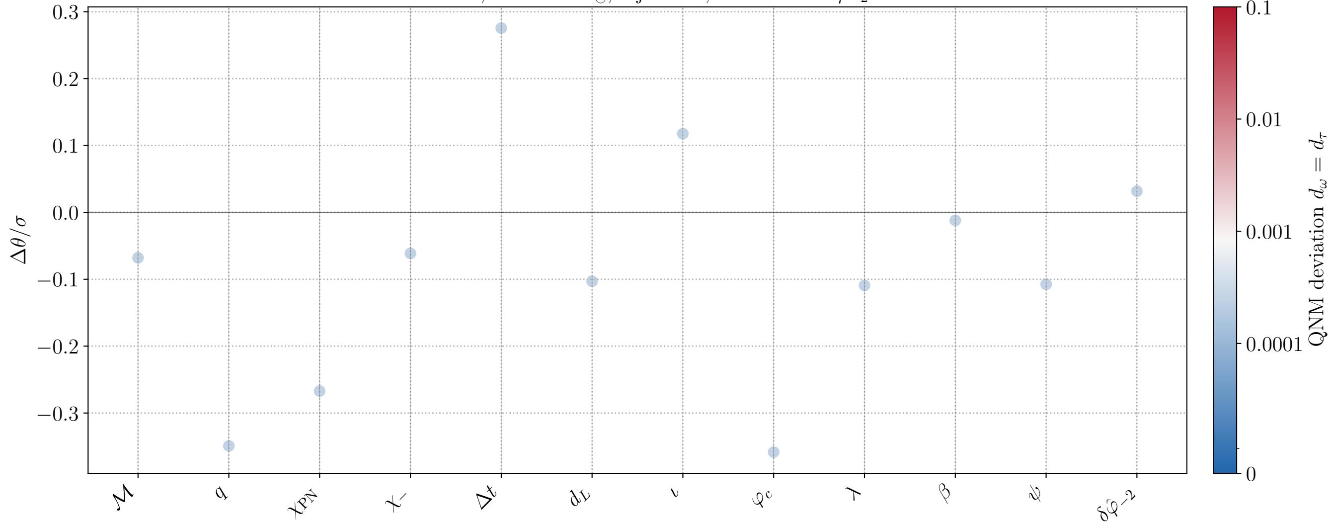
CV bias, M = 10^6 M_\odot , inj_id=12, active FTI: \delta\hat{\varphi}_{-2}
