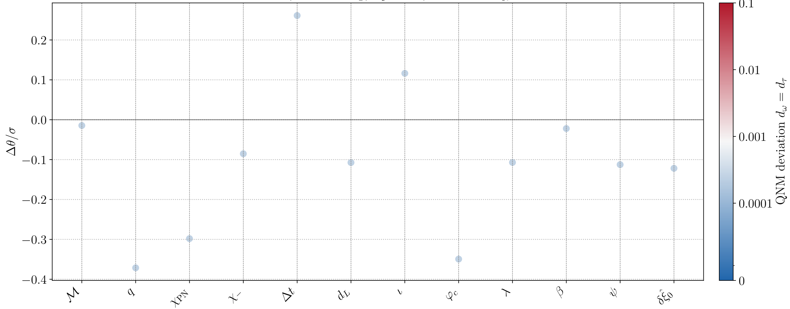
CV bias, M = 10^6 M_\odot , inj_id=12, active FTI: \delta\hat{\xi}_0
