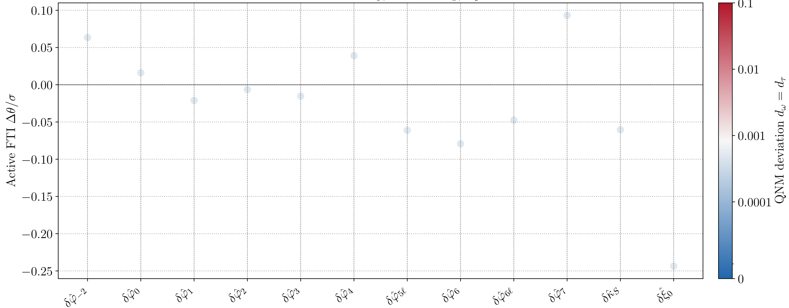
Active-FTI bias summary, M = 10^6 M_\odot , inj_id=13
