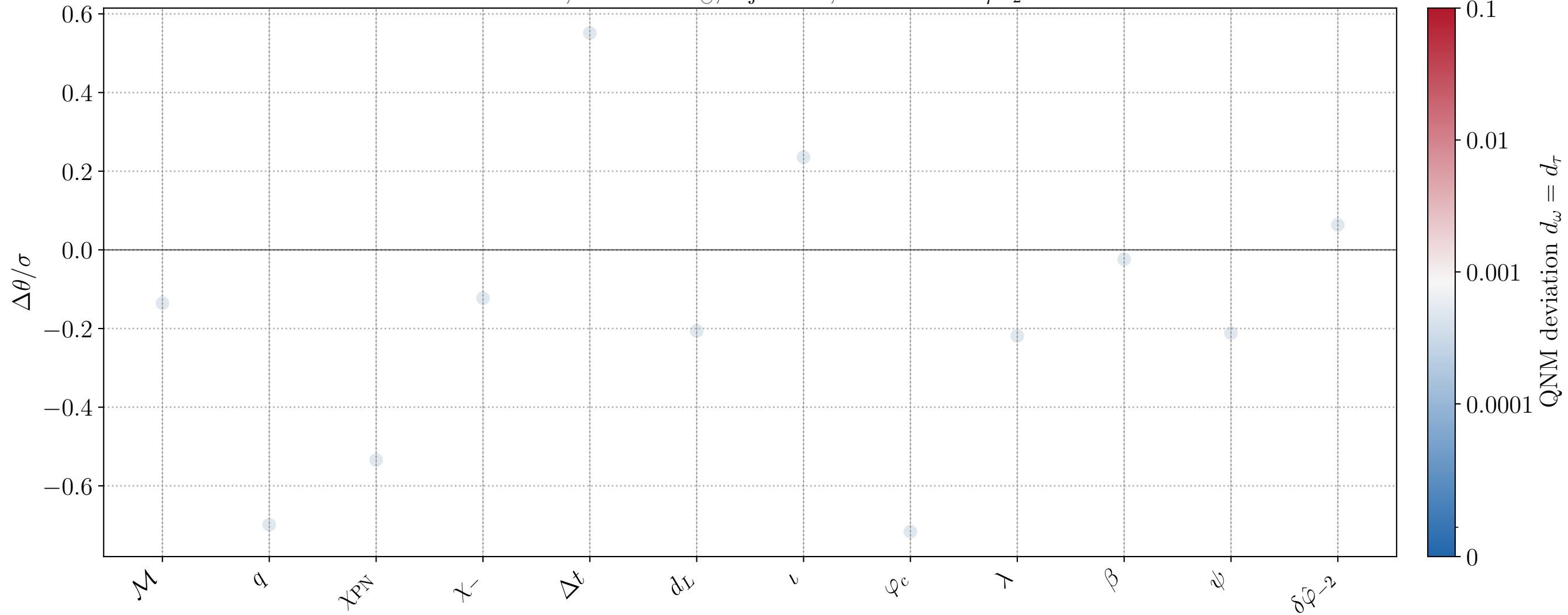
CV bias, M = 10^6 M_\odot , inj_id=13, active FTI: \delta\hat{\varphi}_{-2}
