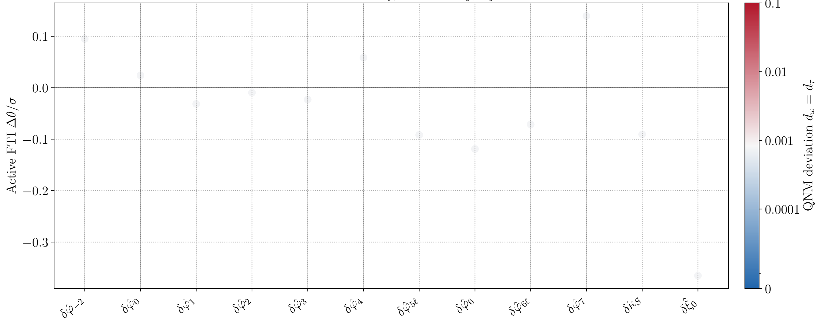
Active-FTI bias summary, M = 10^6 M_\odot , inj_id=14
