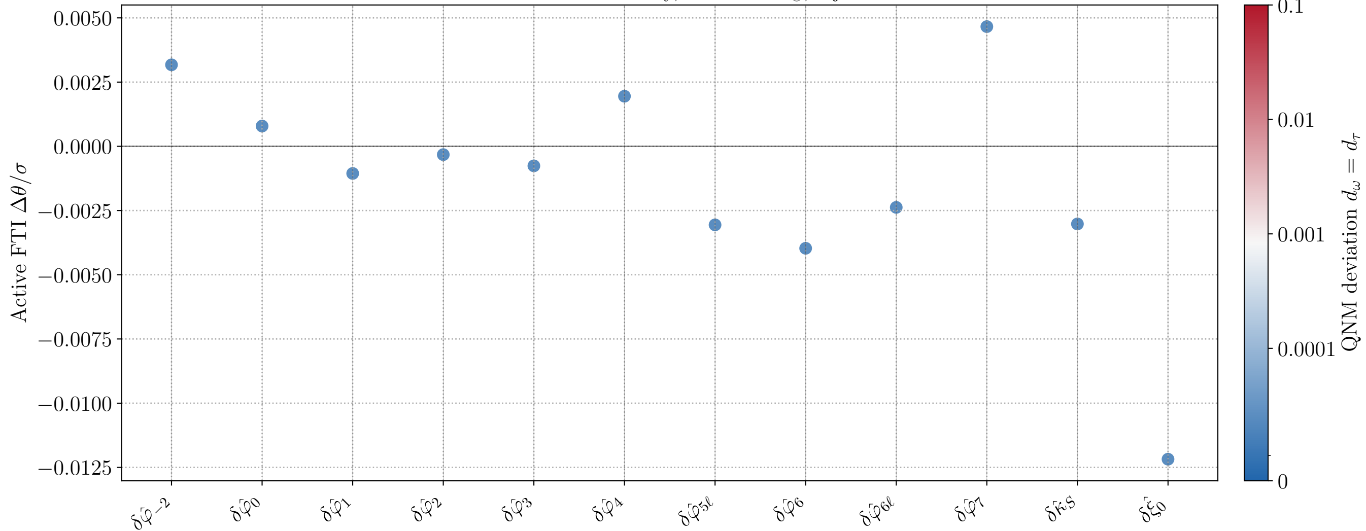
Active-FTI bias summary, M = 10^6 M_\odot , inj_id=15
