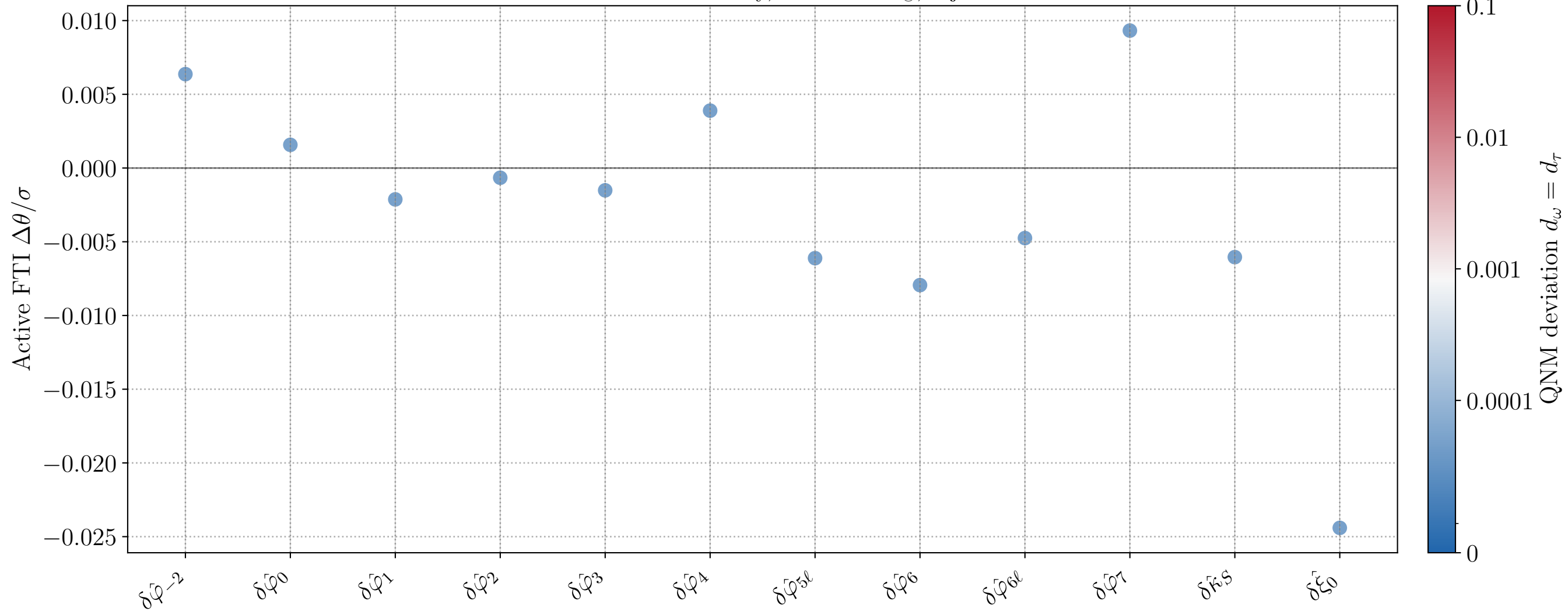
Active-FTI bias summary, M = 10^6 M_\odot , inj_id=16
