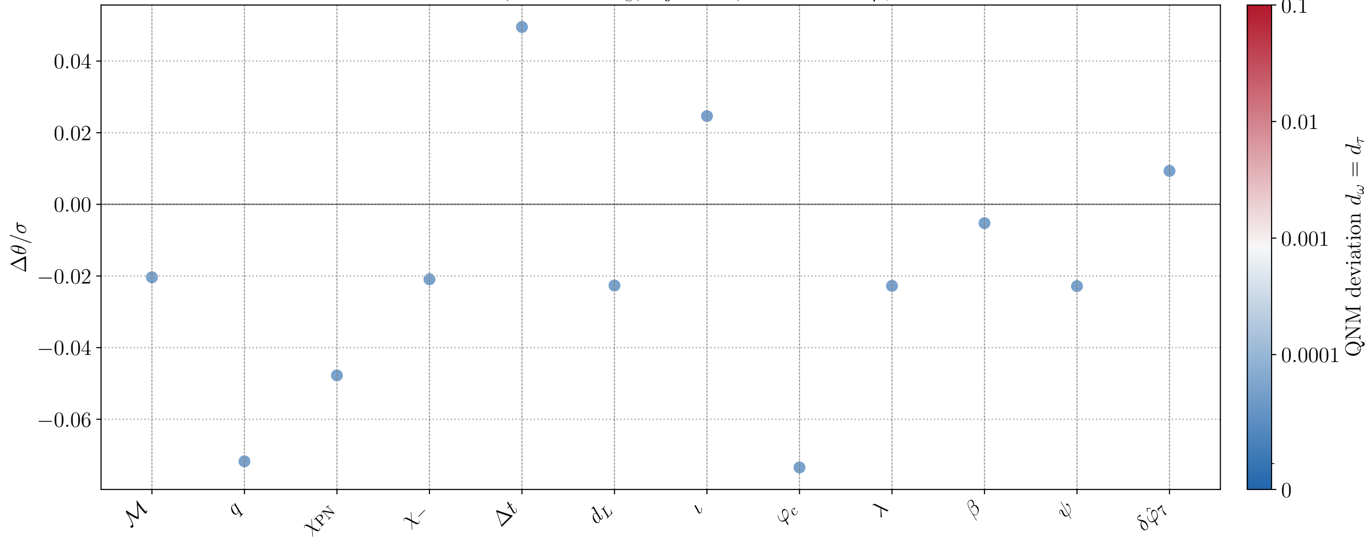
CV bias, M = 10^6 M_\odot , inj_id=16, active FTL: \delta\hat{\varphi}_7
