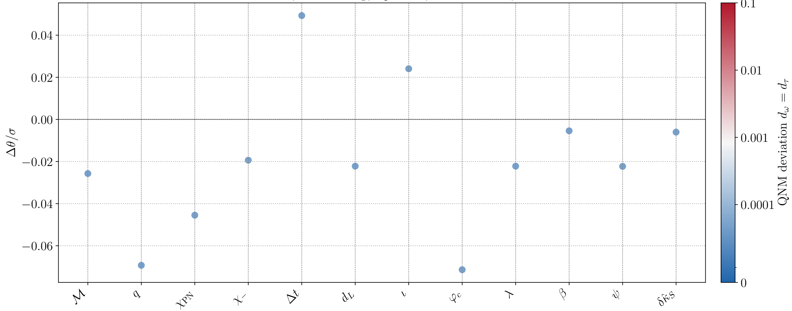
CV bias, M = 10^6 M_\odot , inj_id=16, active FTL: \delta\hat{\kappa}_S
