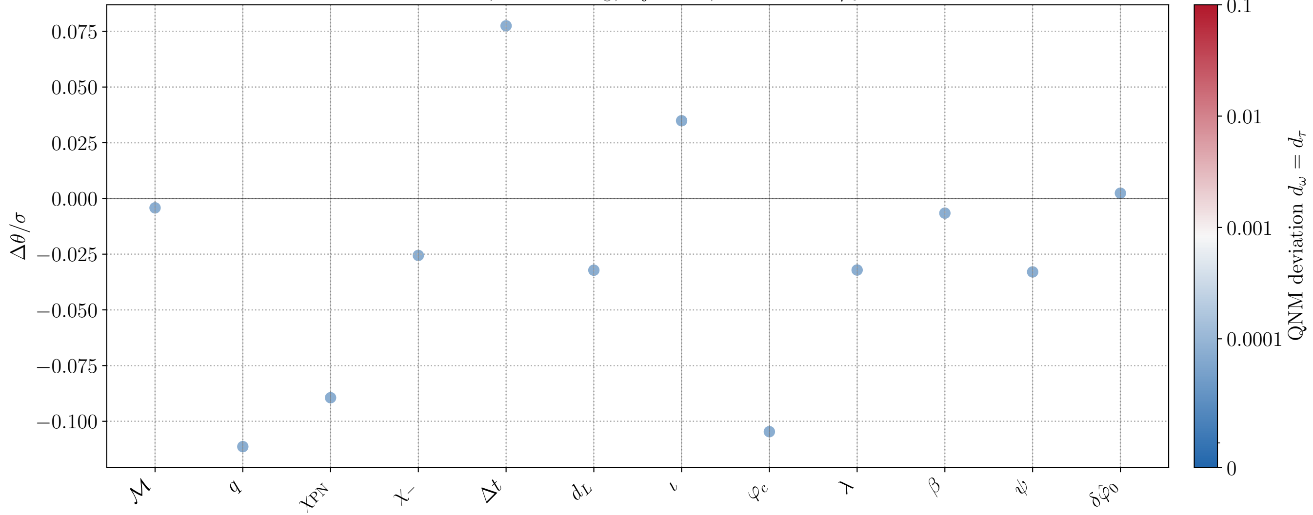
CV bias, M = 10^6 M_\odot , inj_id=17, active FTI: \delta\hat{\varphi}_0
