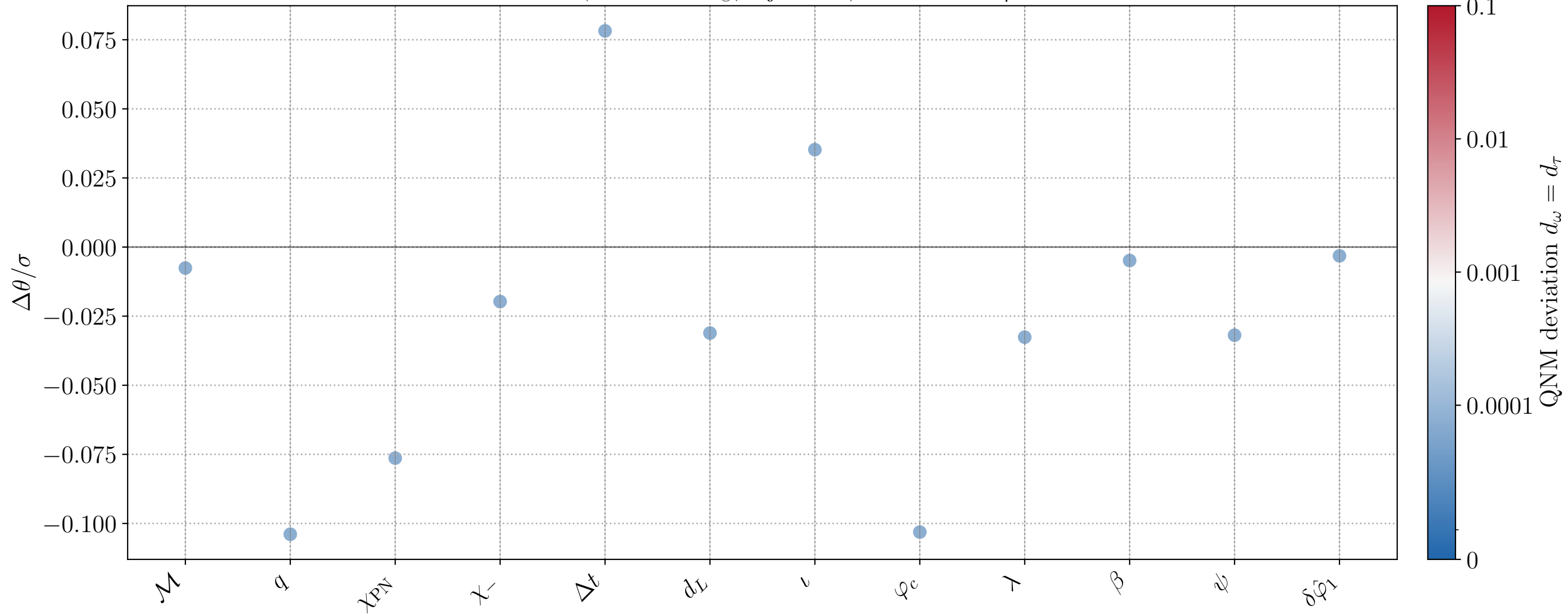
CV bias, M = 10^6 M_\odot , inj_id=17, active FTI: \delta\hat{\varphi}_1
