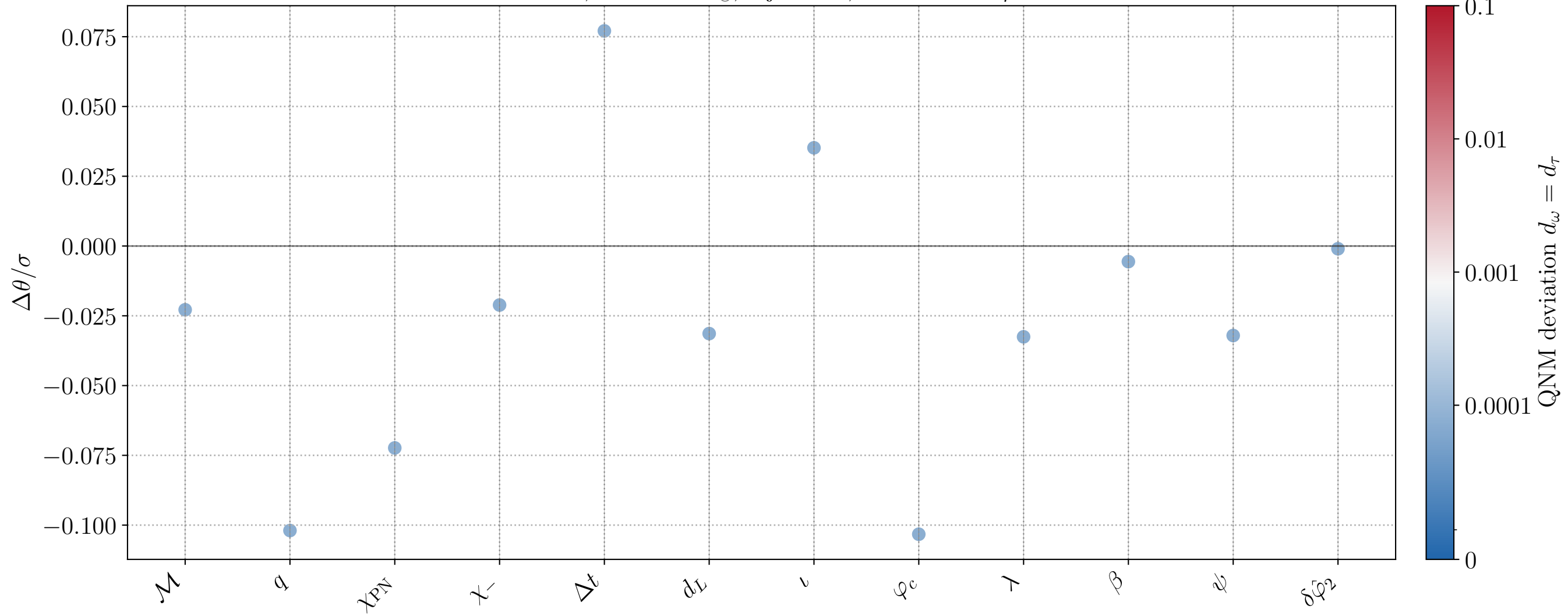
CV bias, M = 10^6 M_\odot , inj_id=17, active FTI: \delta\hat{\varphi}_2
