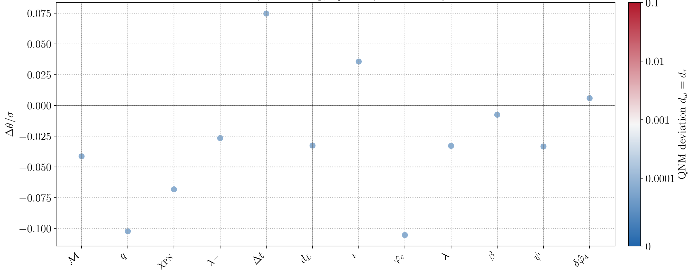
CV bias, M = 10^6 M_\odot , inj_id=17, active FTI: \delta\hat{\varphi}_4
