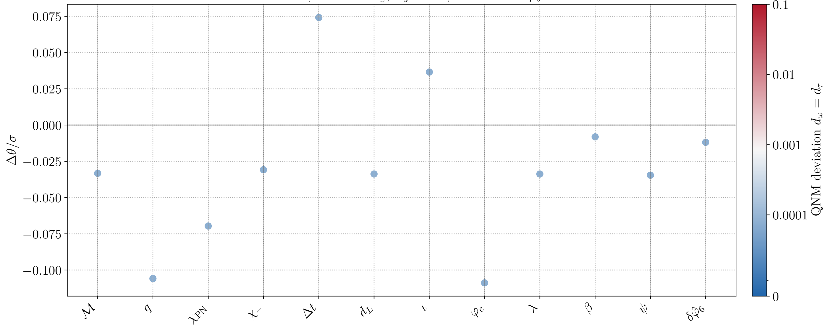
CV bias, M = 10^6 M_\odot , inj_id=17, active FTI: \delta\hat{\varphi}_6
