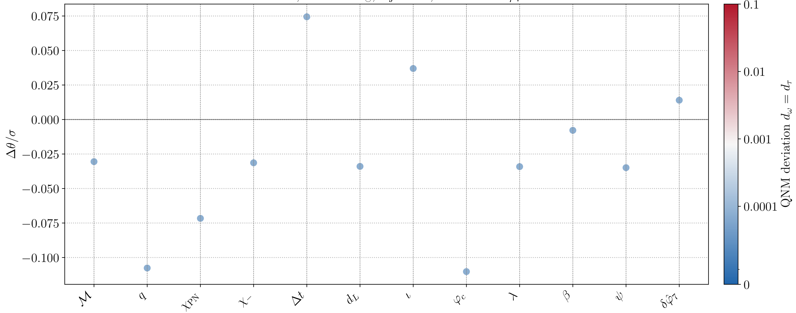
CV bias, M = 10^6 M_\odot , inj_id=17, active FTI: \delta\hat{\varphi}_7
