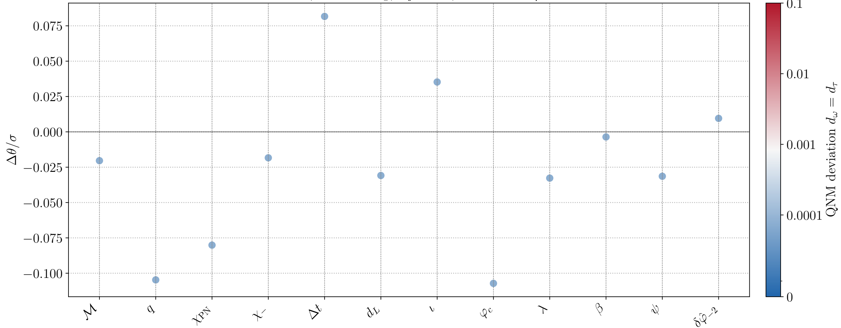
CV bias, M = 10^6 M_\odot , inj_id=17, active FTL: \delta\hat{\varphi}_{-2}
