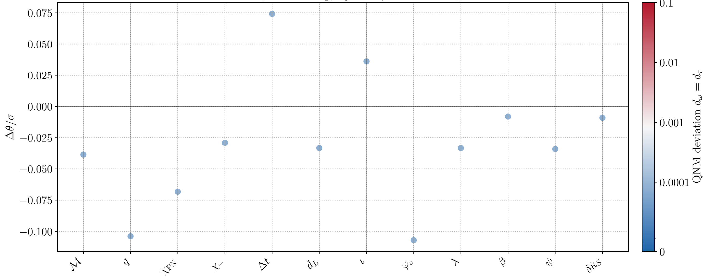
CV bias, M = 10^6 M_\odot , inj_id=17, active FTI: \delta\hat{\kappa}_S
