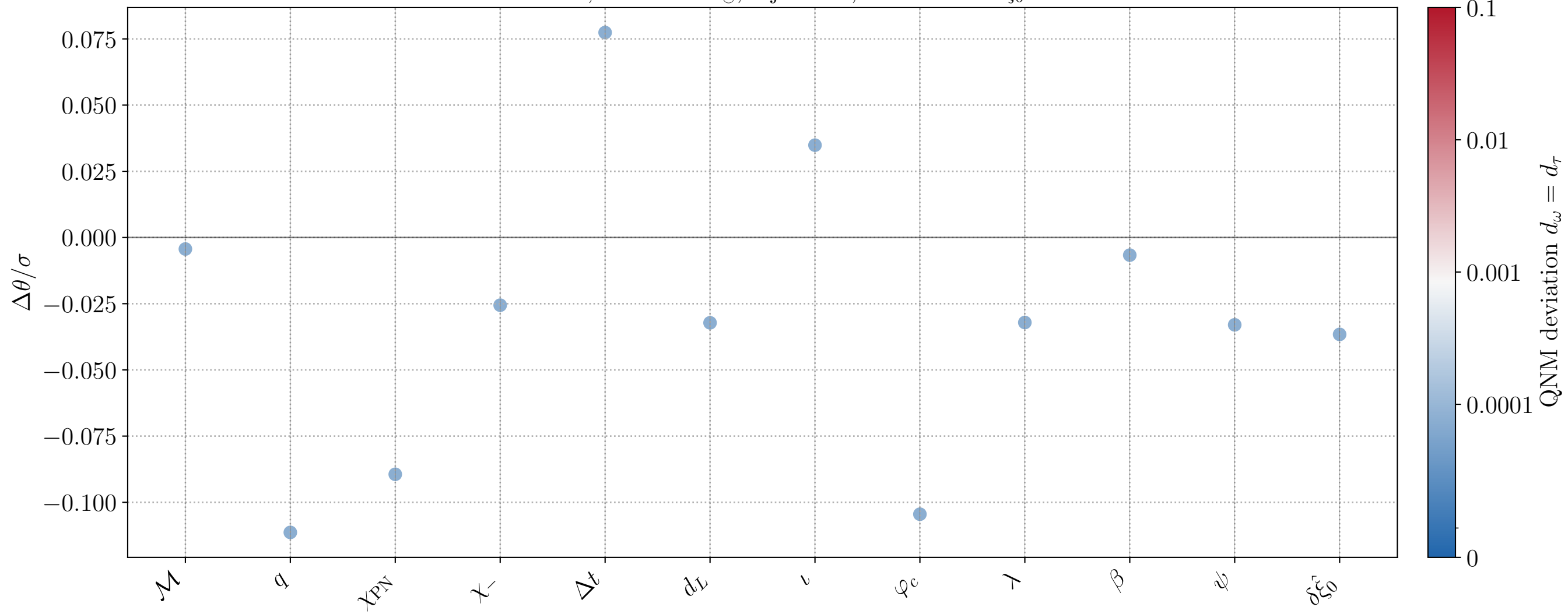
CV bias, M = 10^6 M_\odot , inj_id=17, active FTI: \delta\hat{\xi}_0
