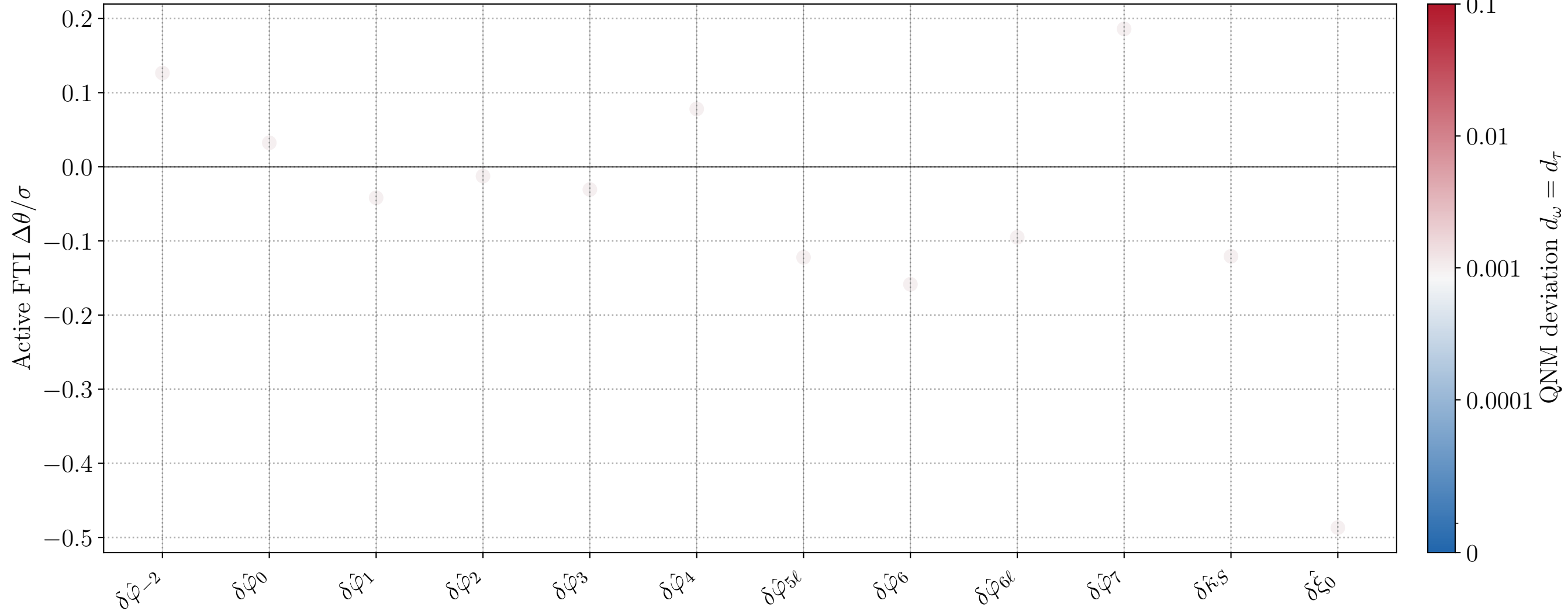
Active-FTI bias summary, M = 10^6 M_\odot , inj_id=2
