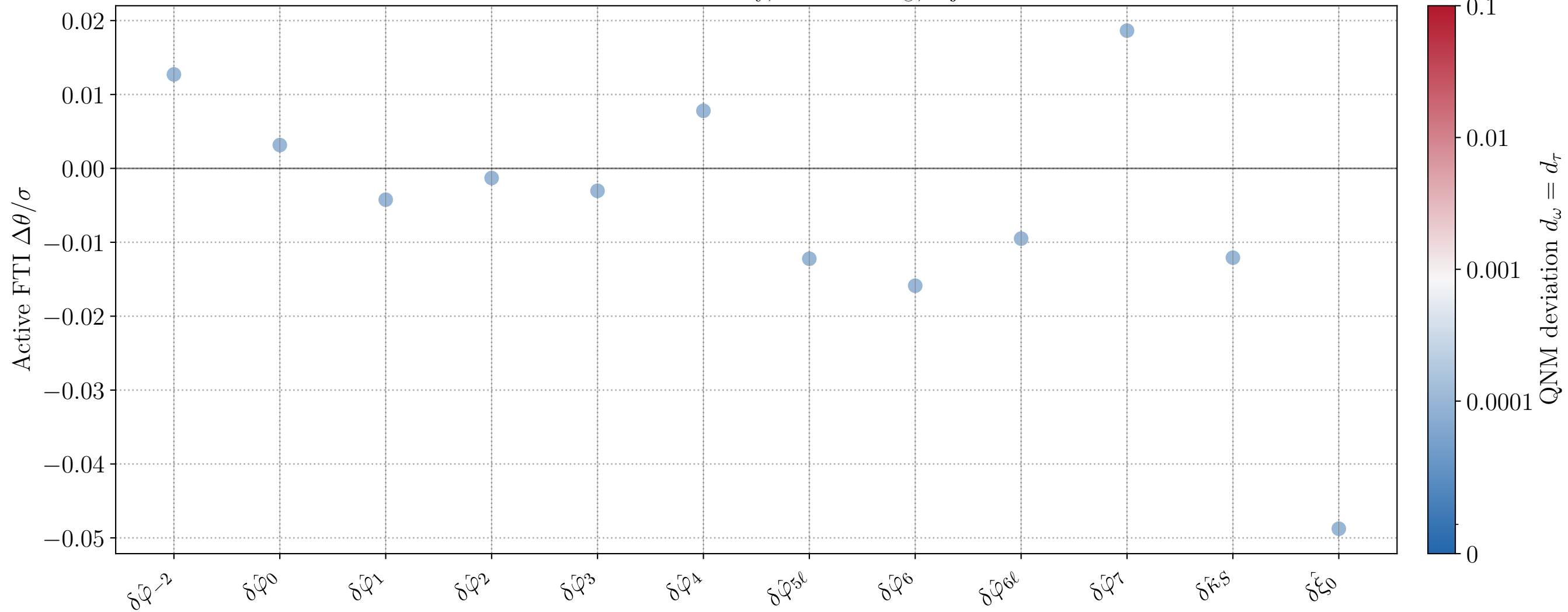
Active-FTI bias summary, M = 10^6 M_\odot , inj_id=3
