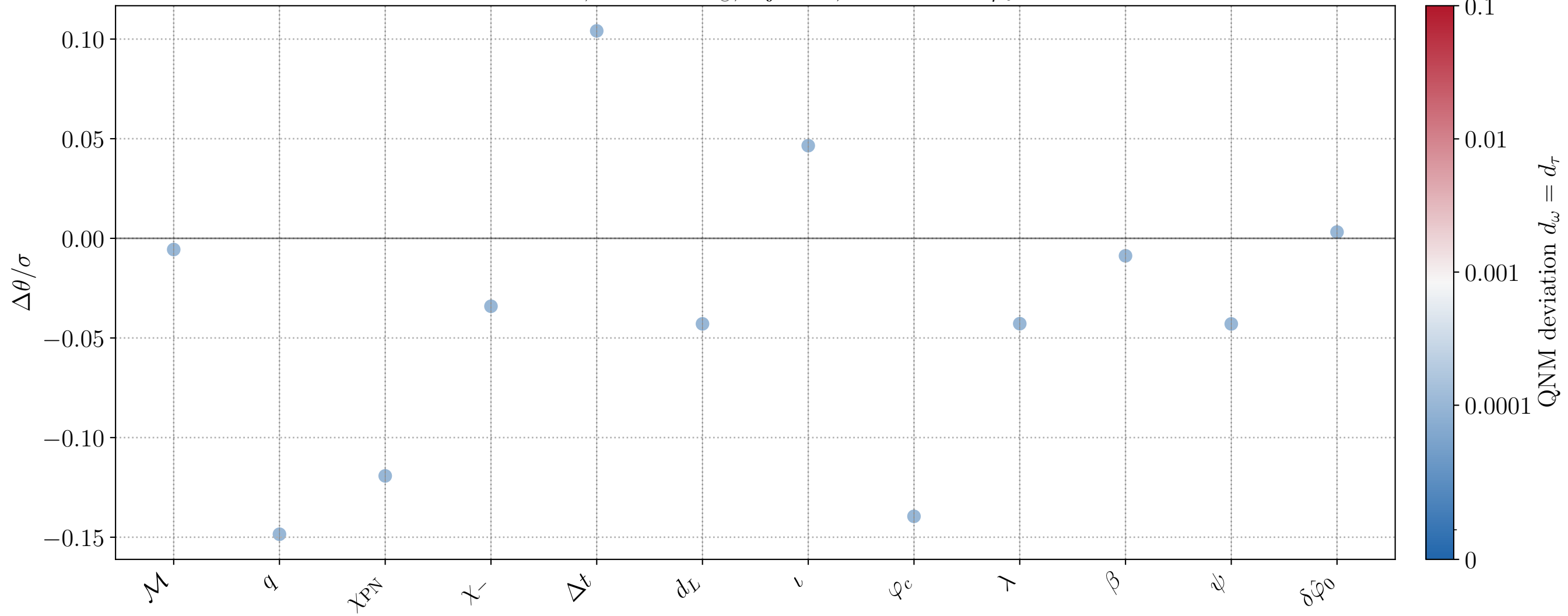
CV bias, M = 10^6 M_\odot , inj_id=3, active FTI: \delta\hat{\varphi}_0
