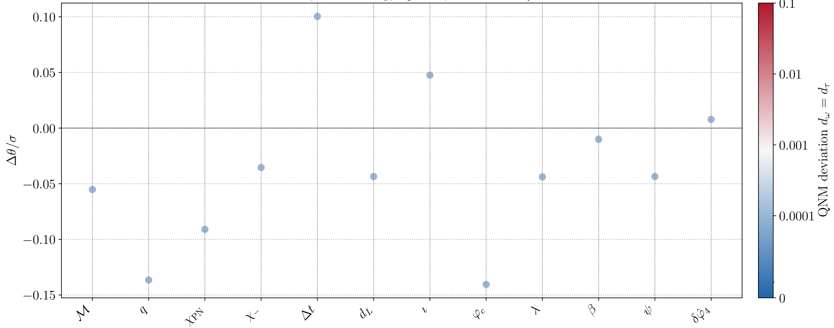
CV bias, M = 10^6 M_\odot , inj_id=3, active FTI: \delta\hat{\varphi}_4
