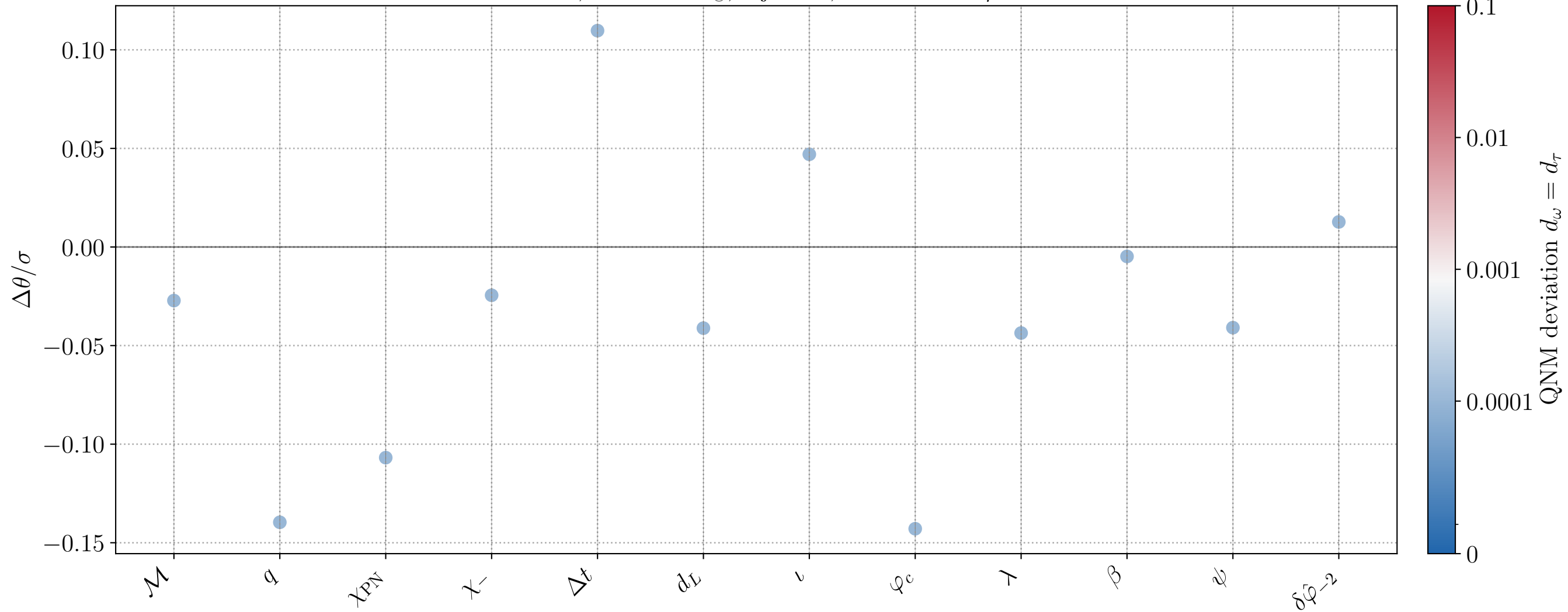
CV bias, M = 10^6 M_\odot , inj_id=3, active FTI: \delta\hat{\varphi}_{-2}
