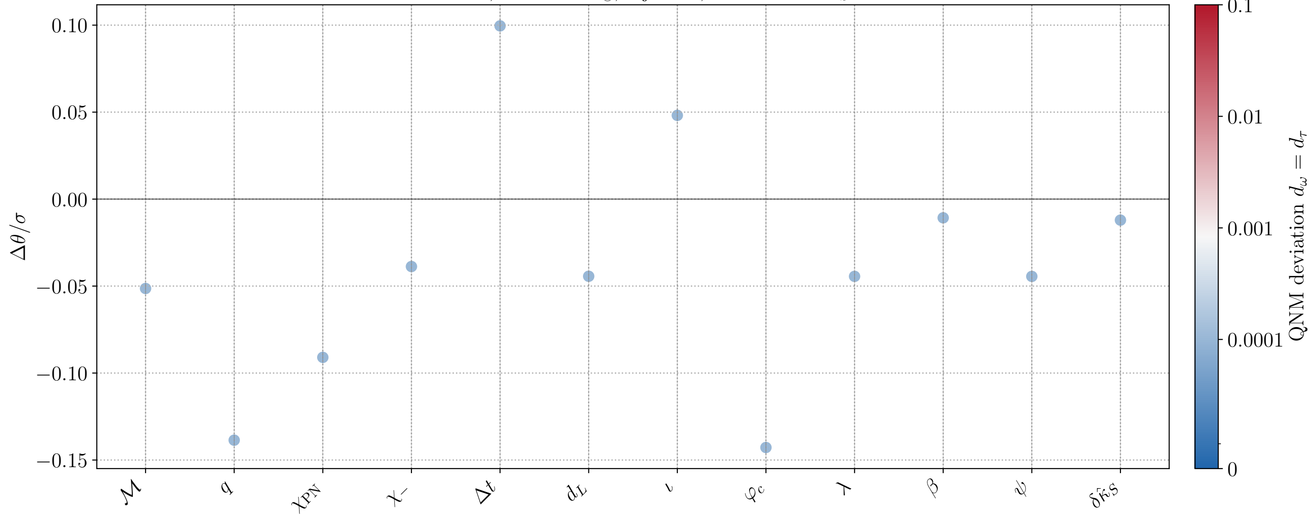
CV bias, M = 10^6 M_\odot , inj_id=3, active FTI: \delta\hat{\kappa}_S
