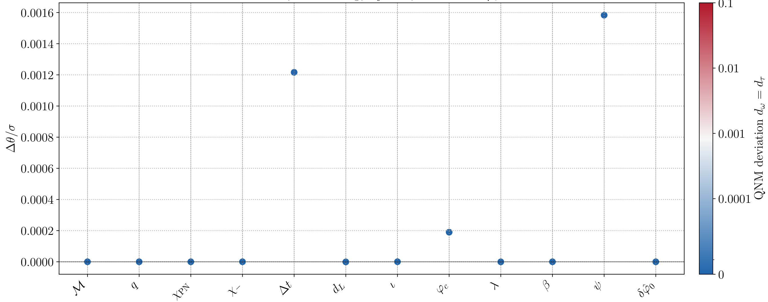
CV bias, M = 10^6 M_\odot , inj_id=4, active FTI: \delta\hat{\varphi}_0
