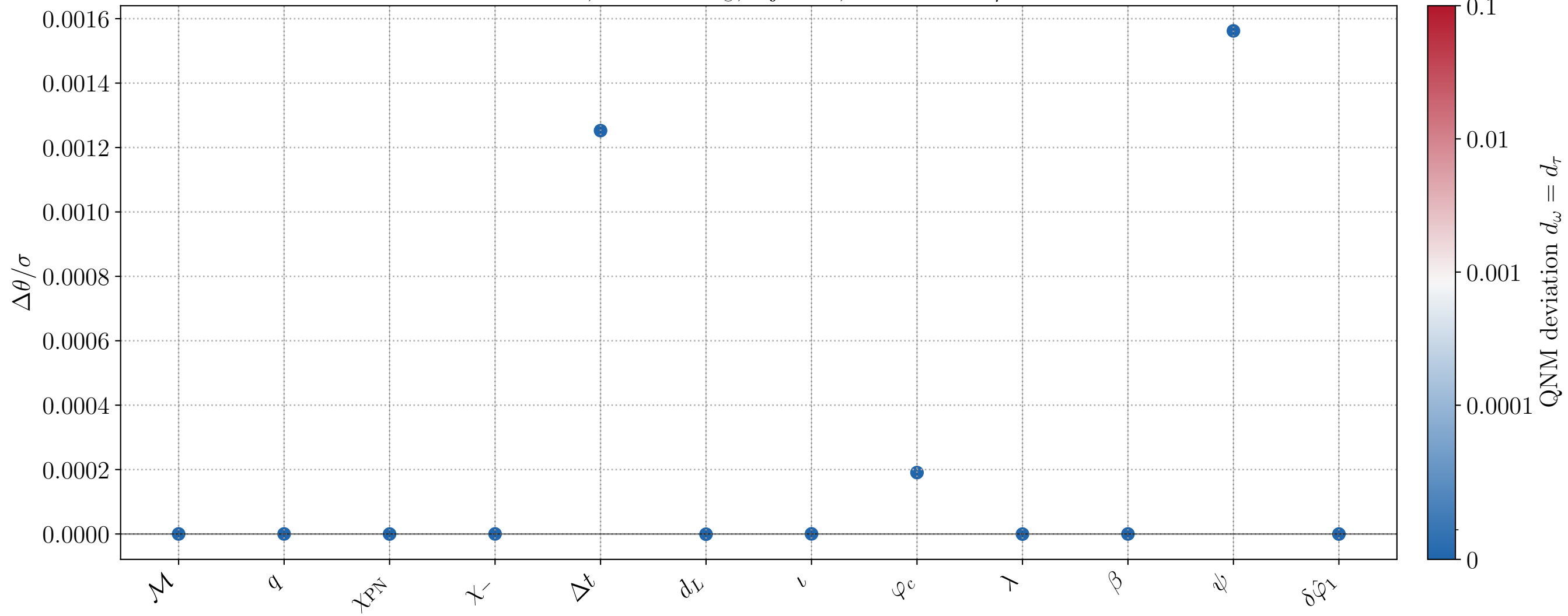
CV bias, M = 10^6 M_\odot , inj_id=4, active FTI: \delta\hat{\varphi}_1
