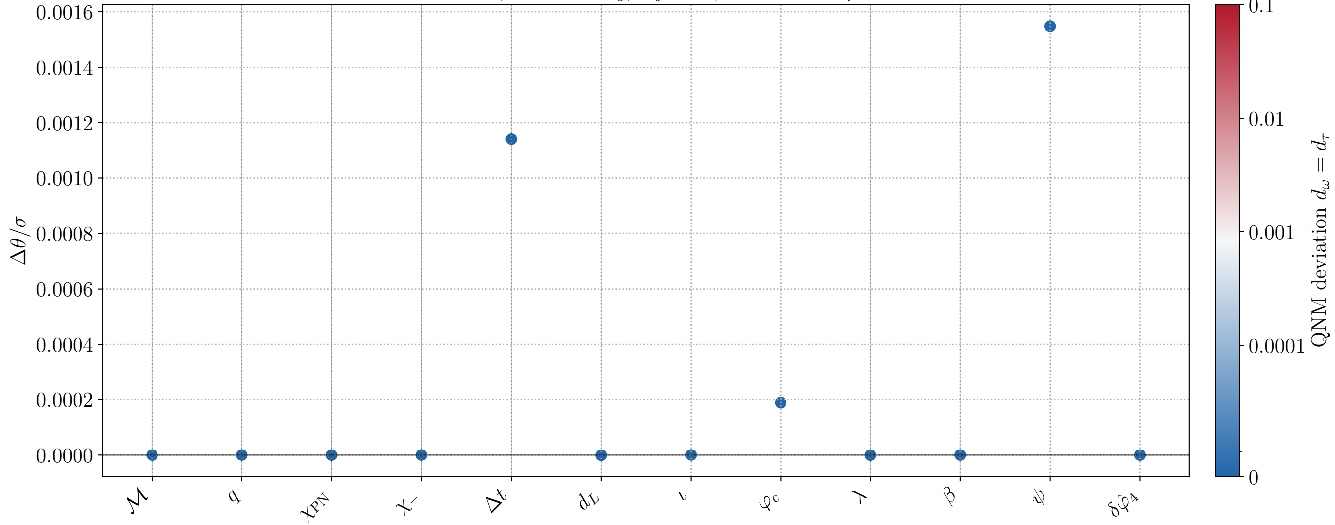
CV bias, M = 10^6 M_\odot , inj_id=4, active FTI: \delta\hat{\varphi}_4
