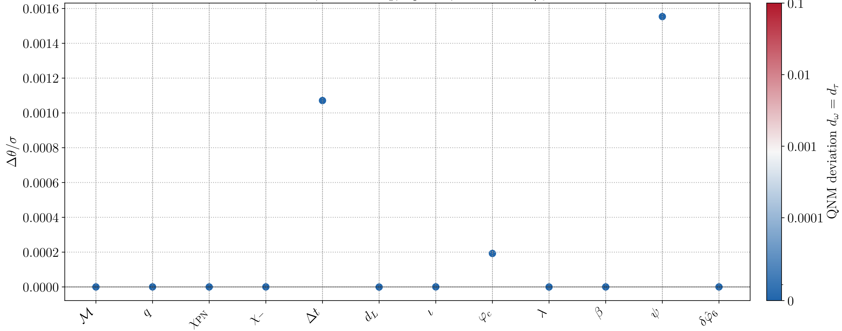
CV bias, M = 10^6 M_\odot , inj_id=4, active FTI: \delta\hat{\varphi}_6
