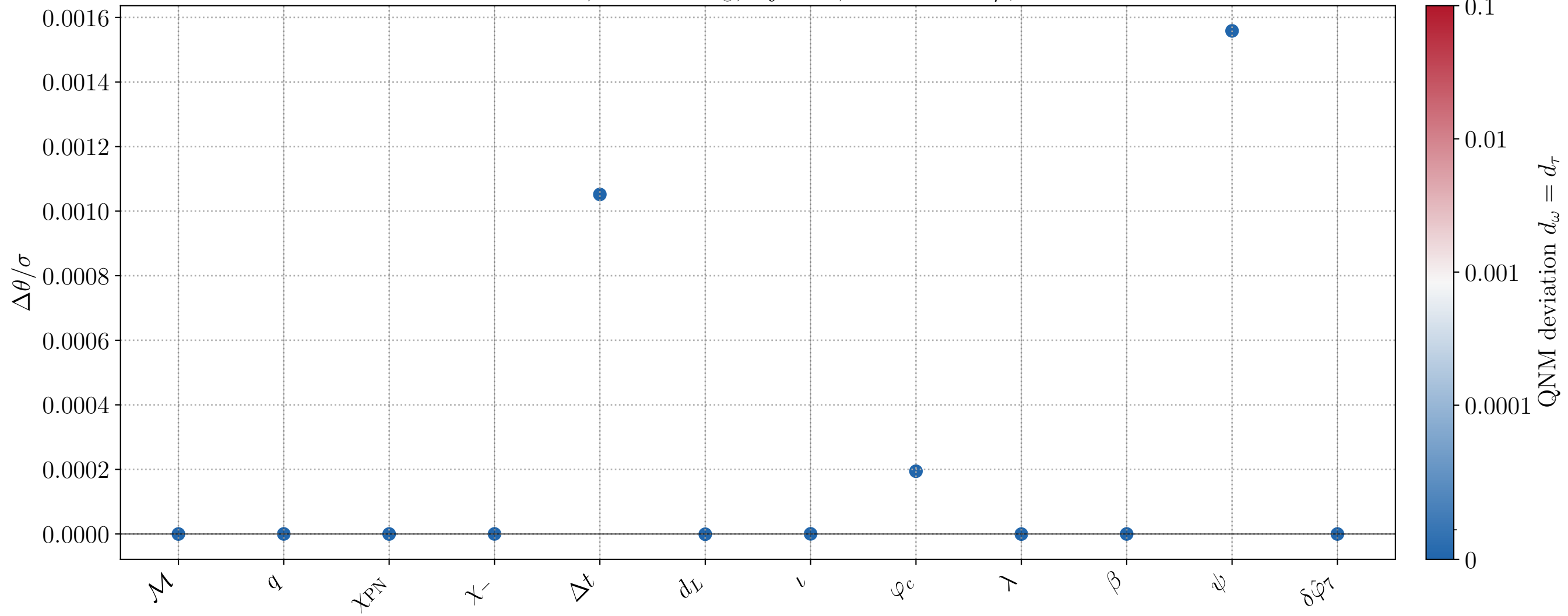
CV bias, M = 10^6 M_\odot , inj_id=4, active FTI: \delta\hat{\varphi}_7
