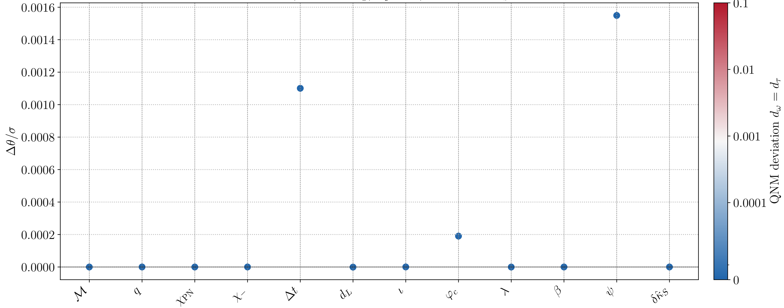
CV bias, M = 10^6 M_\odot , inj_id=4, active FTI: \delta\hat{\kappa}_S
