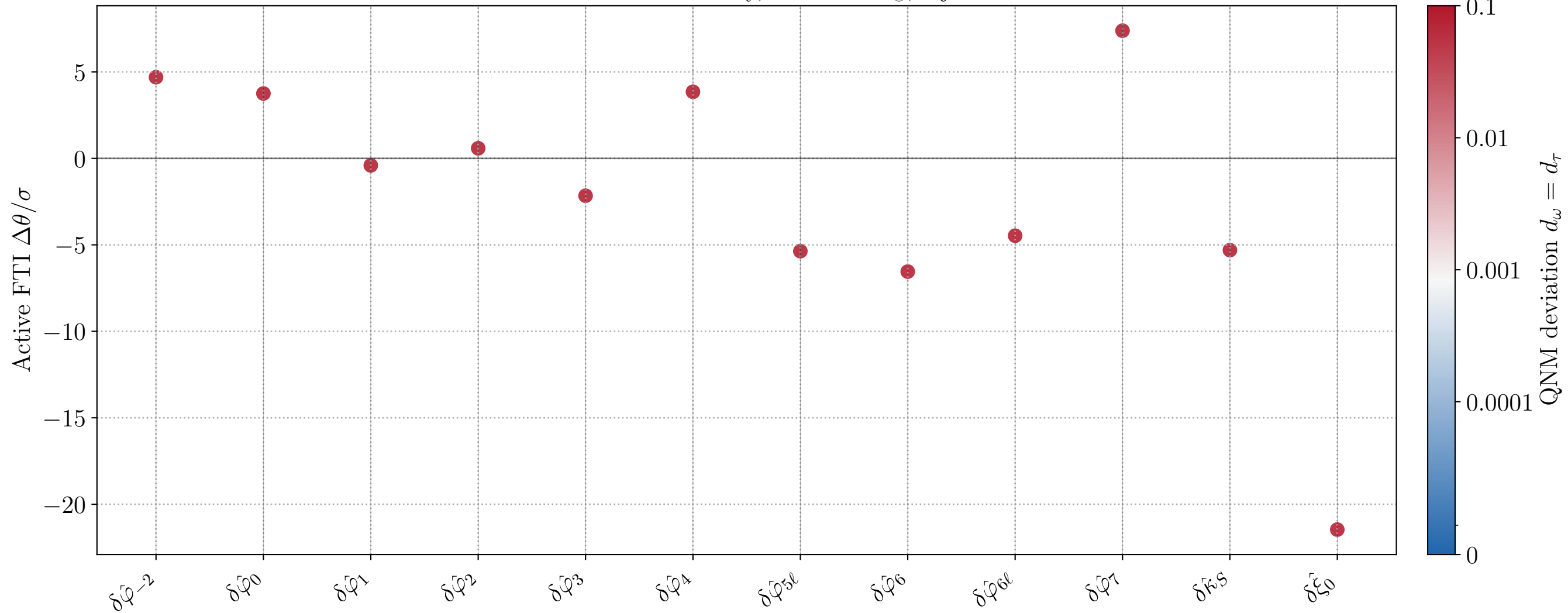
Active-FTI bias summary, M = 10^6 M_\odot , inj_id=5
