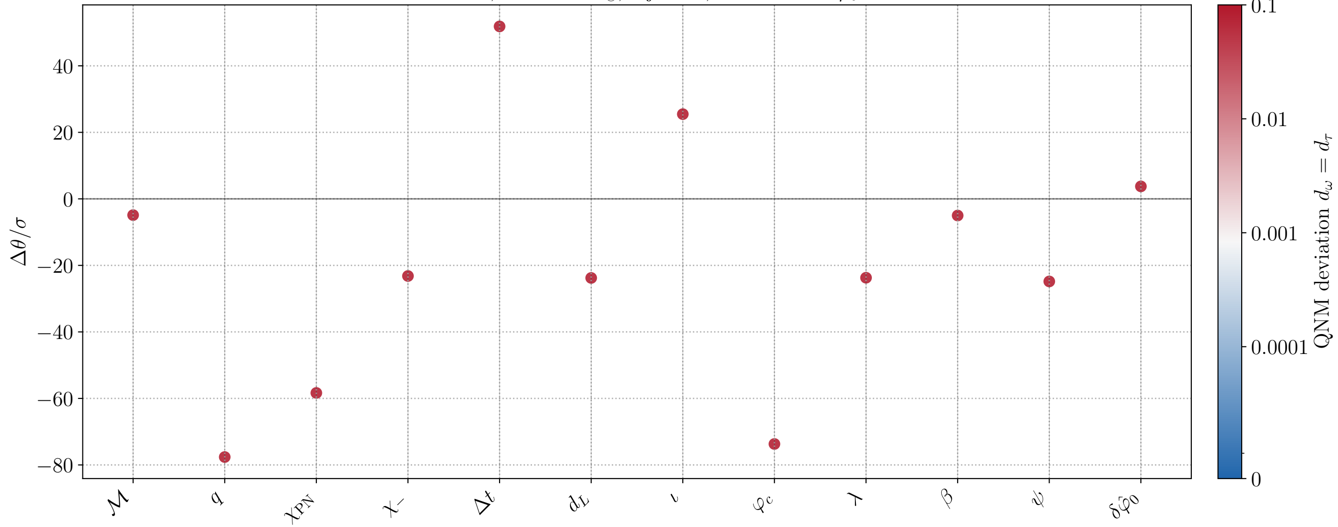
CV bias, M = 10^6 M_\odot , inj_id=5, active FTI: \delta\hat{\varphi}_0
