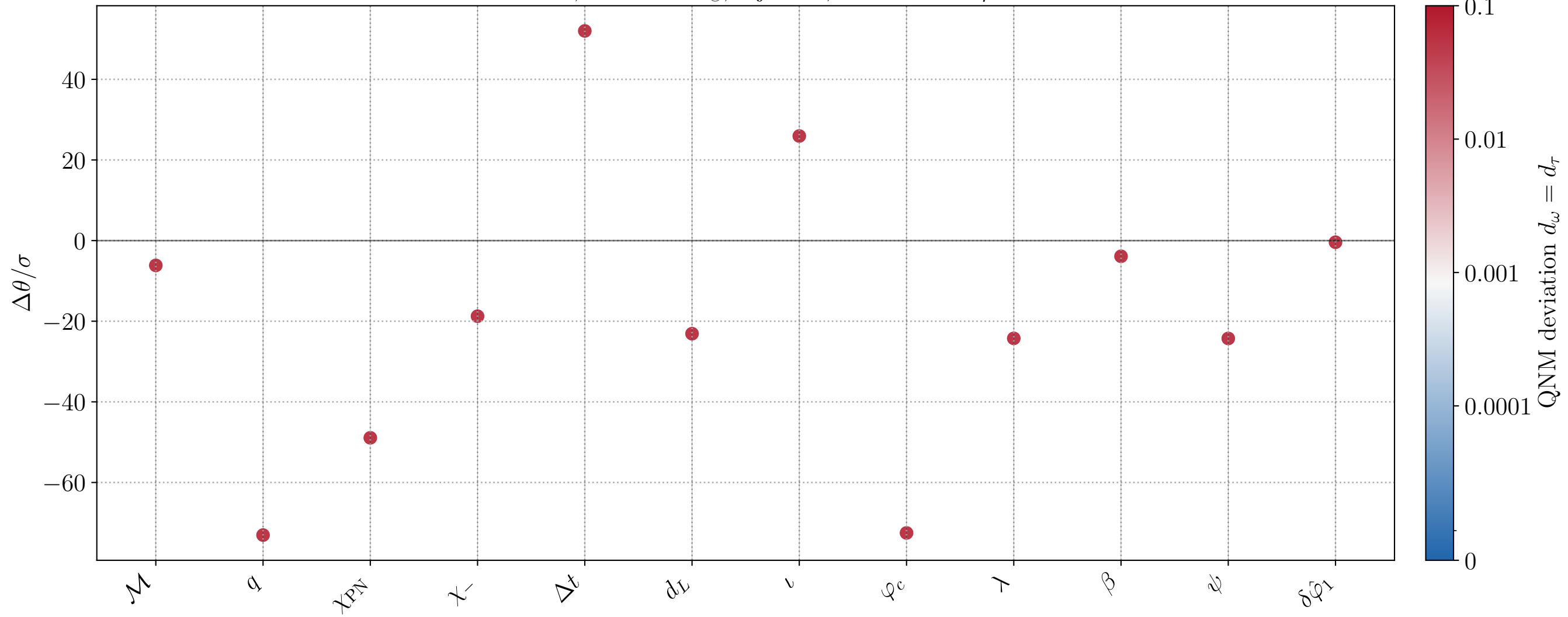
CV bias, M = 10^6 M_\odot , inj_id=5, active FTI: \delta\hat{\varphi}_1
