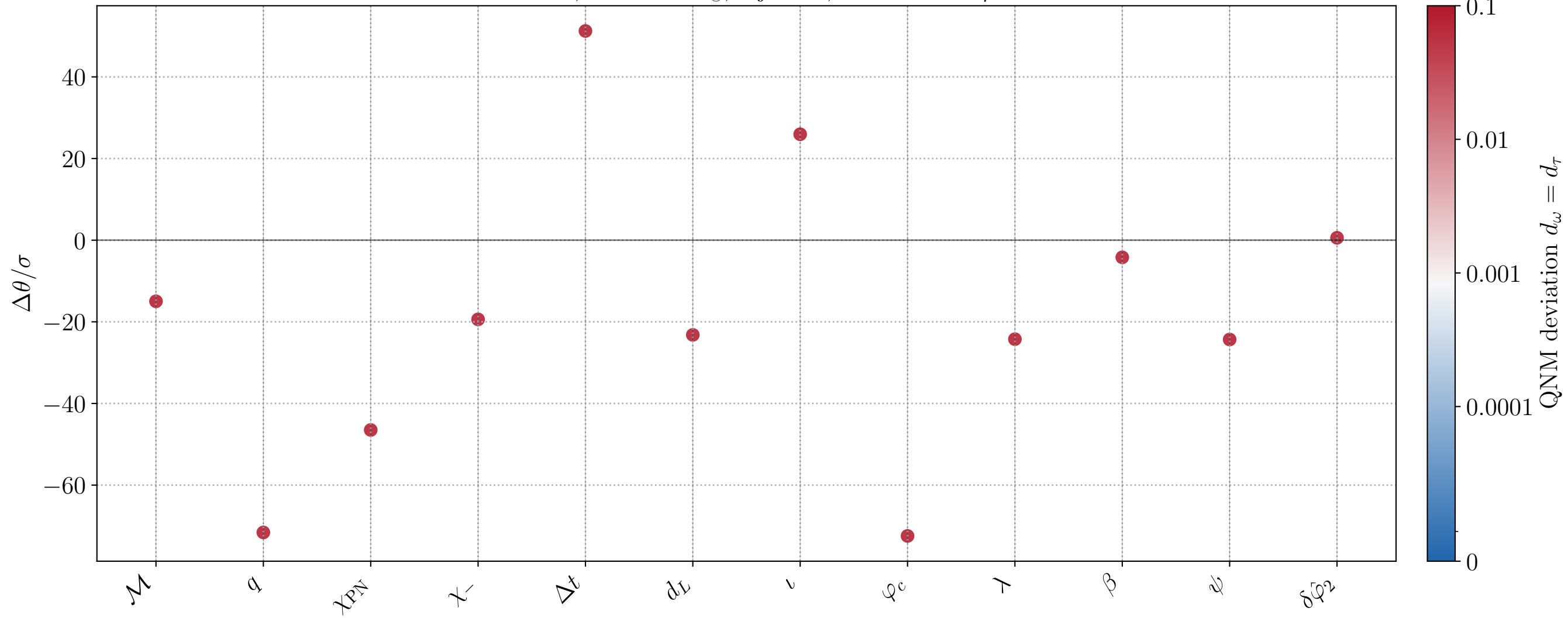
CV bias, M = 10^6 M_\odot , inj_id=5, active FTI: \delta\hat{\varphi}_2
