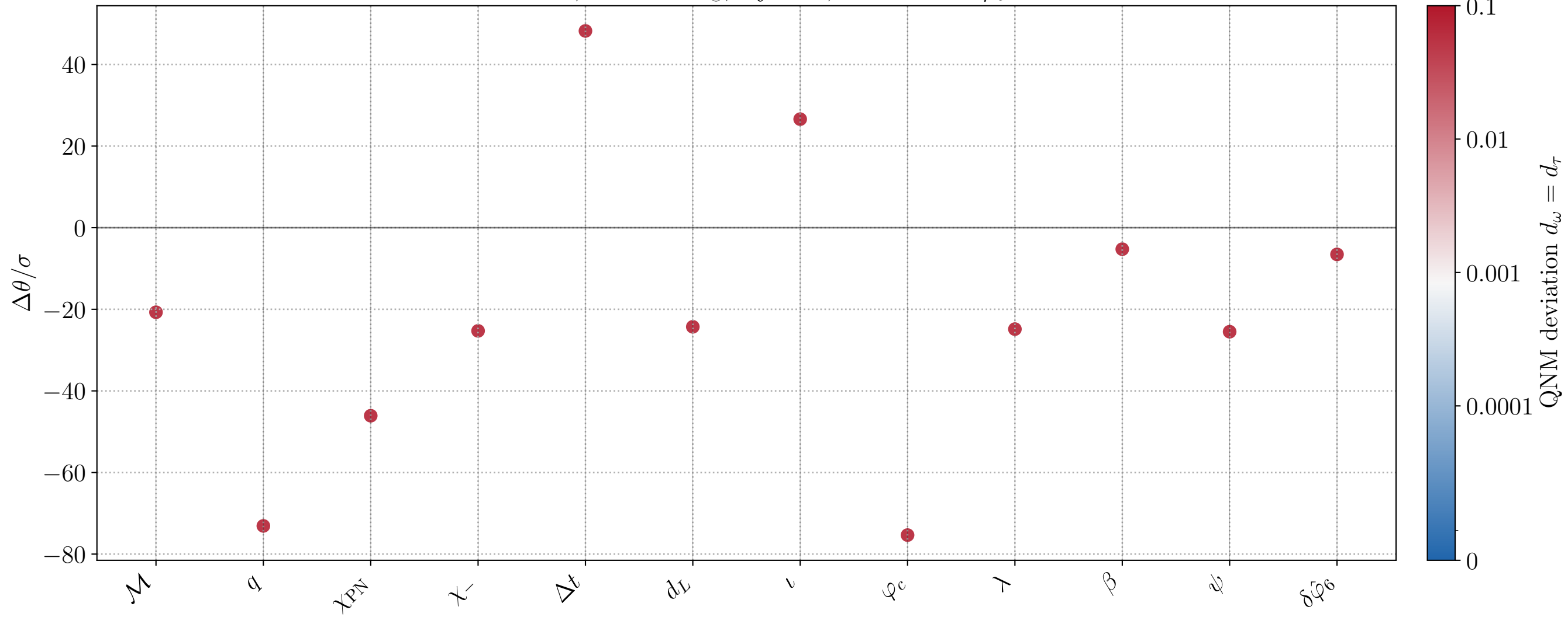
CV bias, M = 10^6 M_\odot , inj_id=5, active FTI: \delta\hat{\varphi}_6
