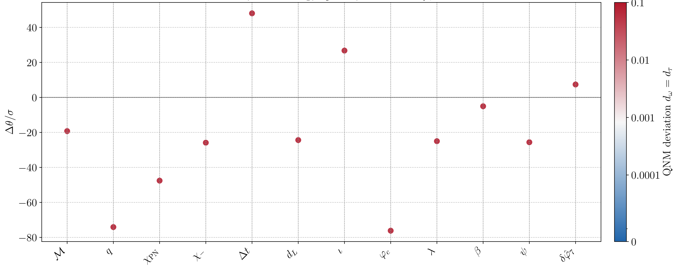
CV bias, M = 10^6 M_\odot , inj_id=5, active FTI: \delta\hat{\varphi}_7
