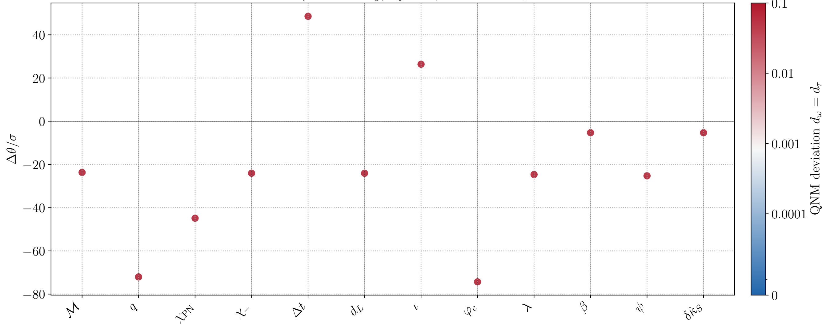
CV bias, M = 10^6 M_\odot , inj_id=5, active FTI: \delta\hat{\kappa}_S
