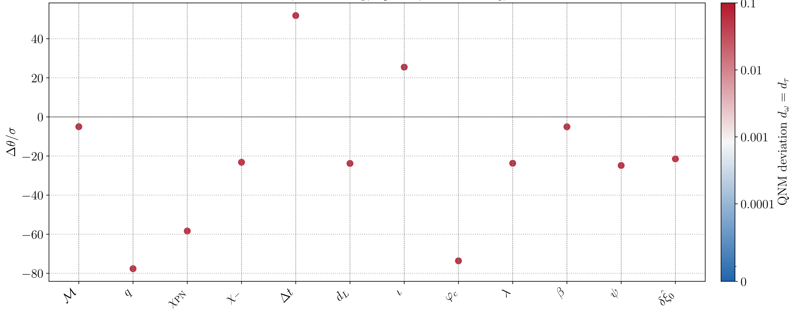
CV bias, M = 10^6 M_\odot , inj_id=5, active FTI: \delta\hat{\xi}_0
