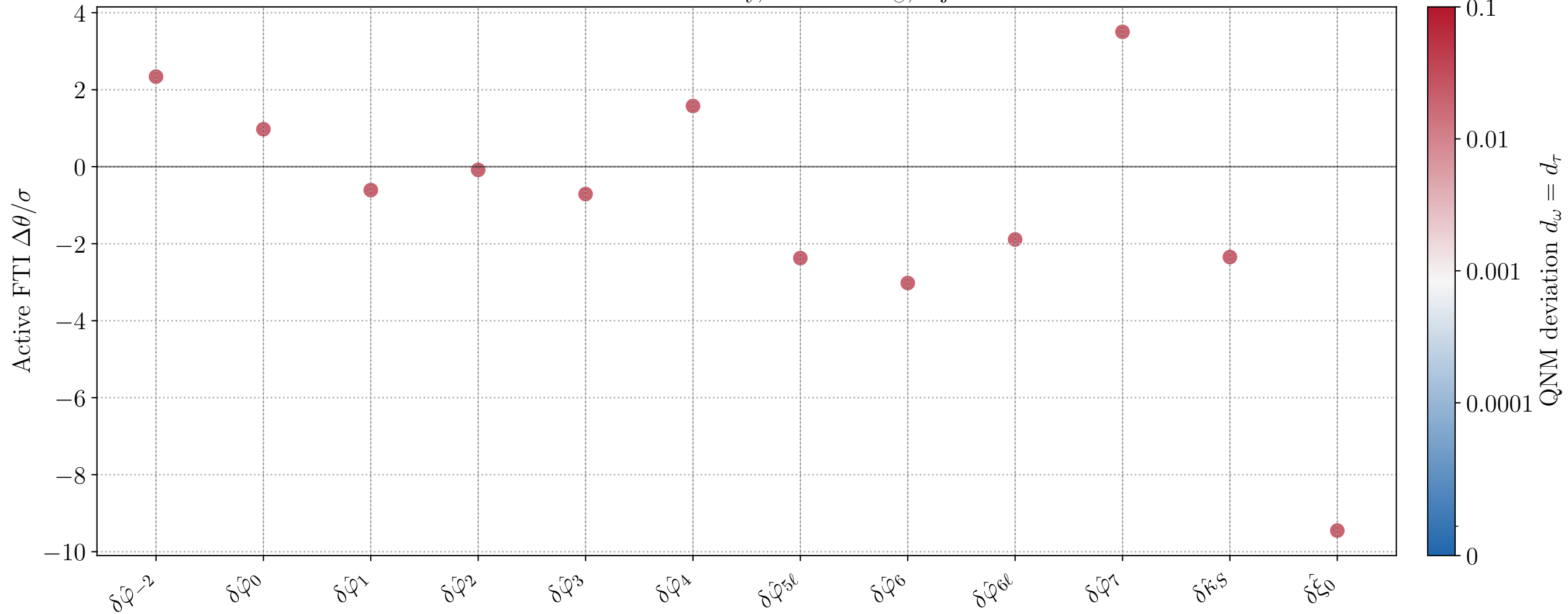
Active-FTI bias summary, M = 10^6 M_\odot , inj_id=6
