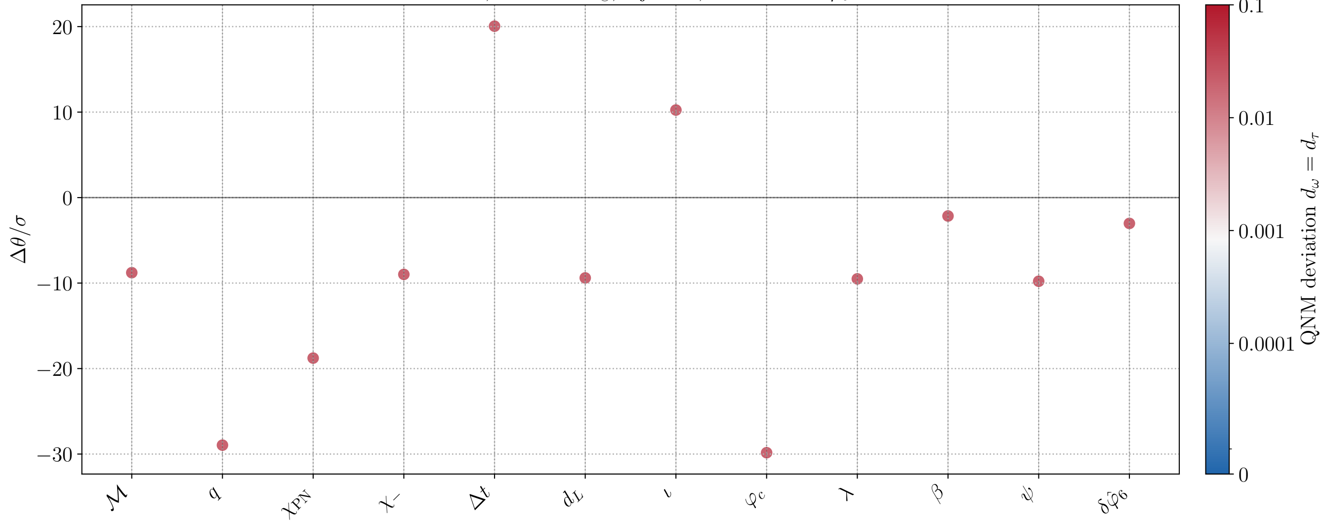
CV bias, M = 10^6 M_\odot , inj_id=6, active FTI: \delta\hat{\varphi}_6
