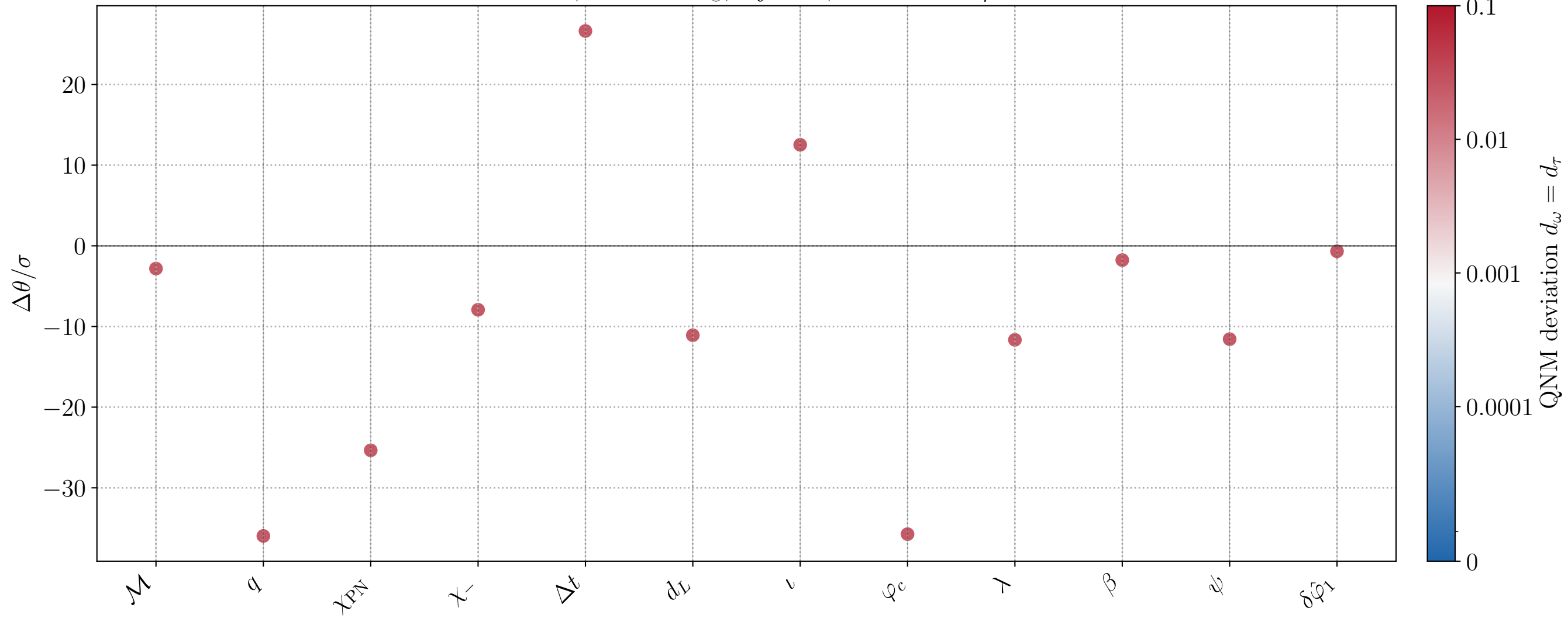
CV bias, M = 10^6 M_\odot , inj_id=7, active FTI: \delta\hat{\varphi}_1
