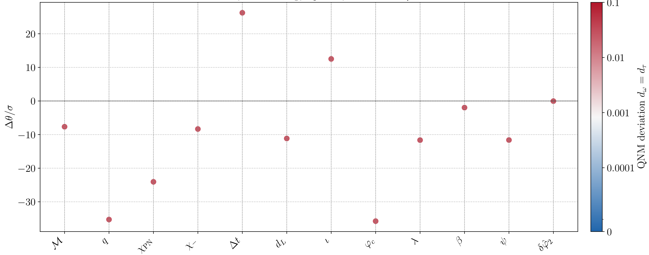
CV bias, M = 10^6 M_\odot , inj_id=7, active FTI: \delta\hat{\varphi}_2
