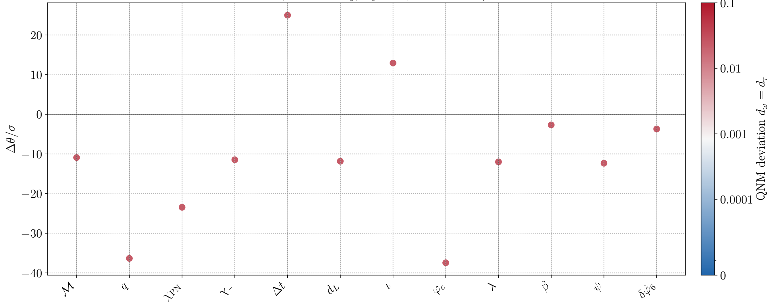
CV bias, M = 10^6 M_\odot , inj_id=7, active FTI: \delta\hat{\varphi}_6
