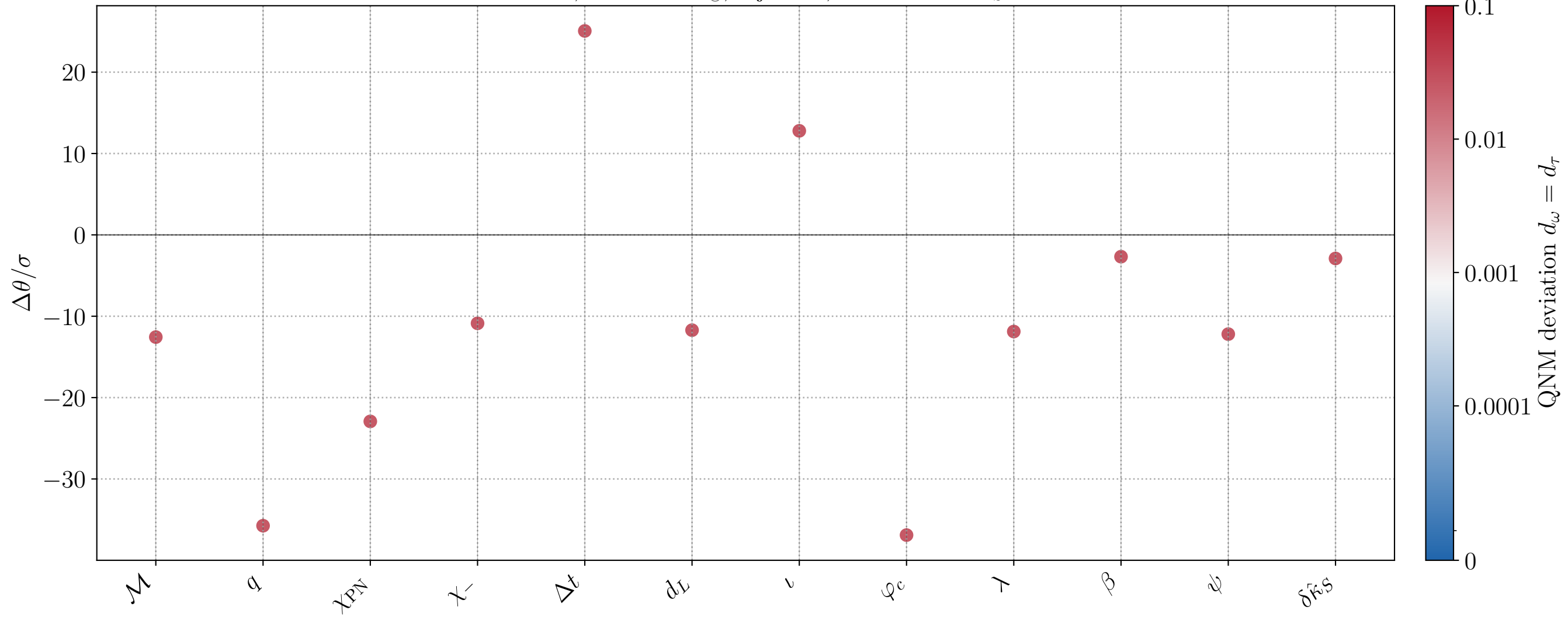
CV bias, M = 10^6 M_\odot , inj_id=7, active FTI: \delta\hat{\kappa}_S
