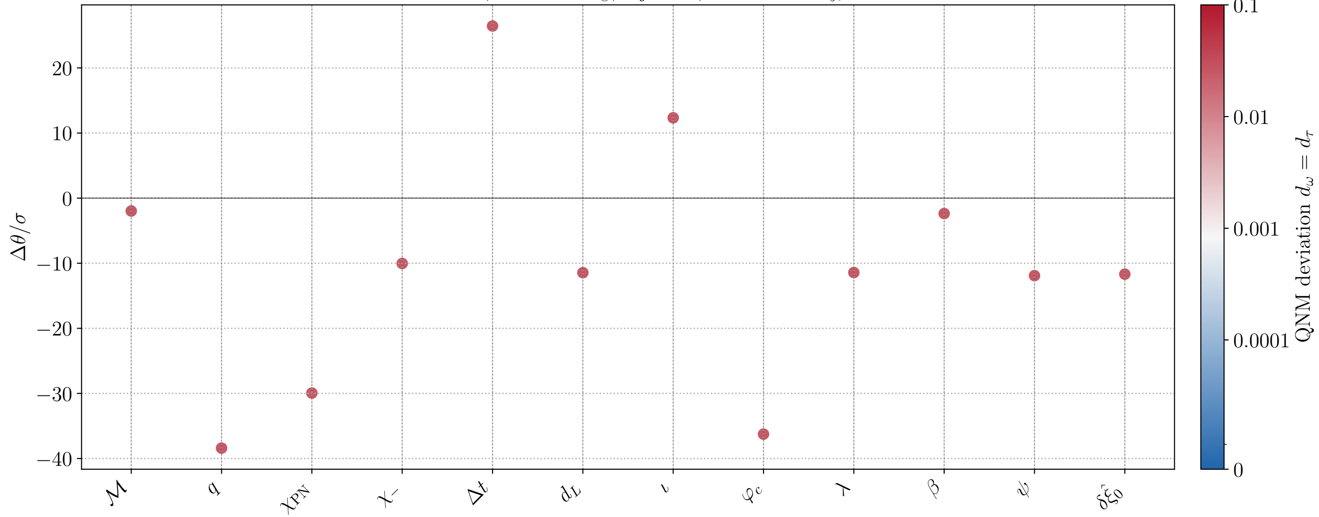
CV bias, M = 10^6 M_\odot , inj_id=7, active FTI: \delta\hat{\xi}_0
