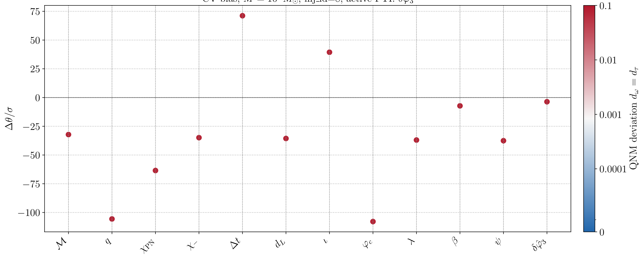
CV bias, M = 10^6 M_\odot , inj_id=8, active FTL: \delta\hat{\varphi}_3
