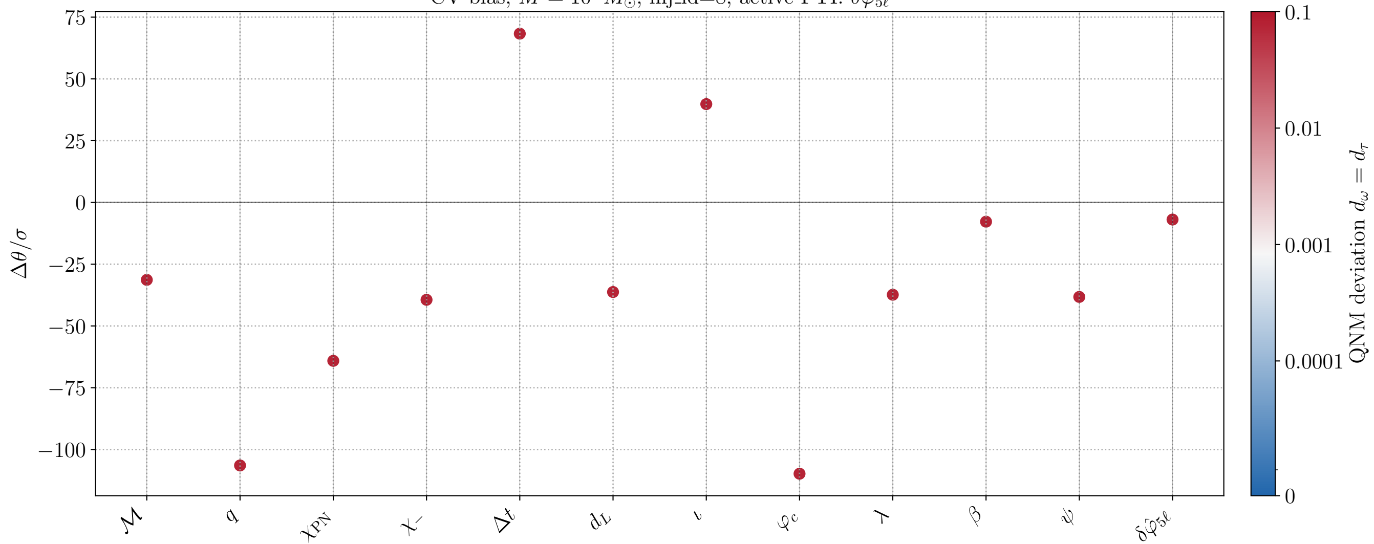
CV bias, M = 10^6 M_\odot , inj_id=8, active FTI: \delta\hat{\varphi}_{5\ell}
